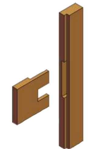
Barefaced tenon joint at mid rail
