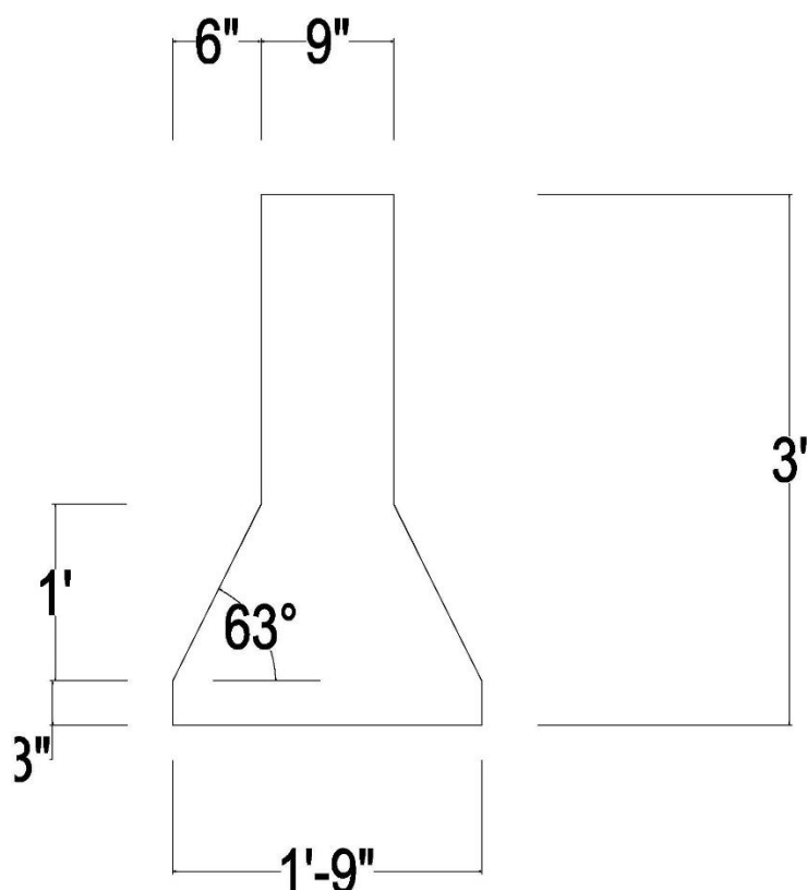
Figure 1 Typical Cross Section of RCC Bridge Railing
