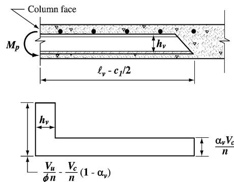
Fig. R11.12.4.5—Idealized shear acting on shearhead
