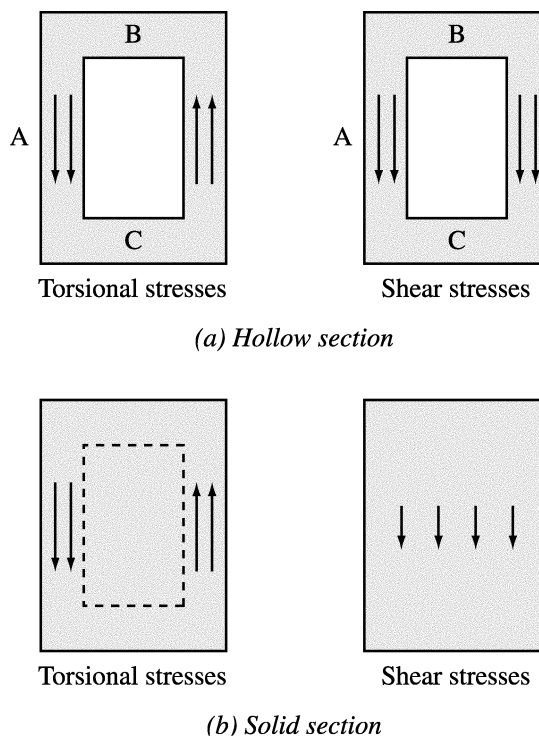
Fig. R11.6.3.1—Addition of torsional and shear stresses
