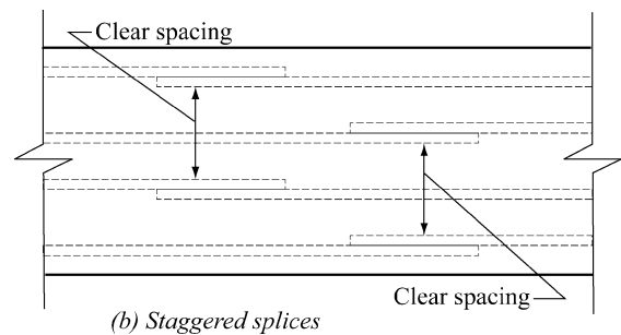
Fig. R12.15.1—Clear spacing of spliced bars
